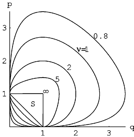
FIG. 1. The phase diagram for type-I scaling. Shown are equi- \nu contours as a function of the mixing parameters.
