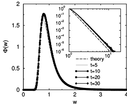
FIG. 3. Self-similarity in type-I scaling. Shown is \Phi(w) versus w for the case p=q=0.4 ( \alpha=0.2 ). In the inset, the tail is compared with the theoretical prediction \nu=4.88636 .
