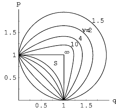
FIG. 2. The phase diagram for type-II scaling.
