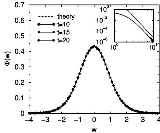
FIG. 4. Self-similarity in type-II scaling. Shown is \Phi(w) versus w for the case p=q=0.6 ( \alpha=0.14 ). The inset compares the tail with the theoretical prediction \nu=6.66937 .
